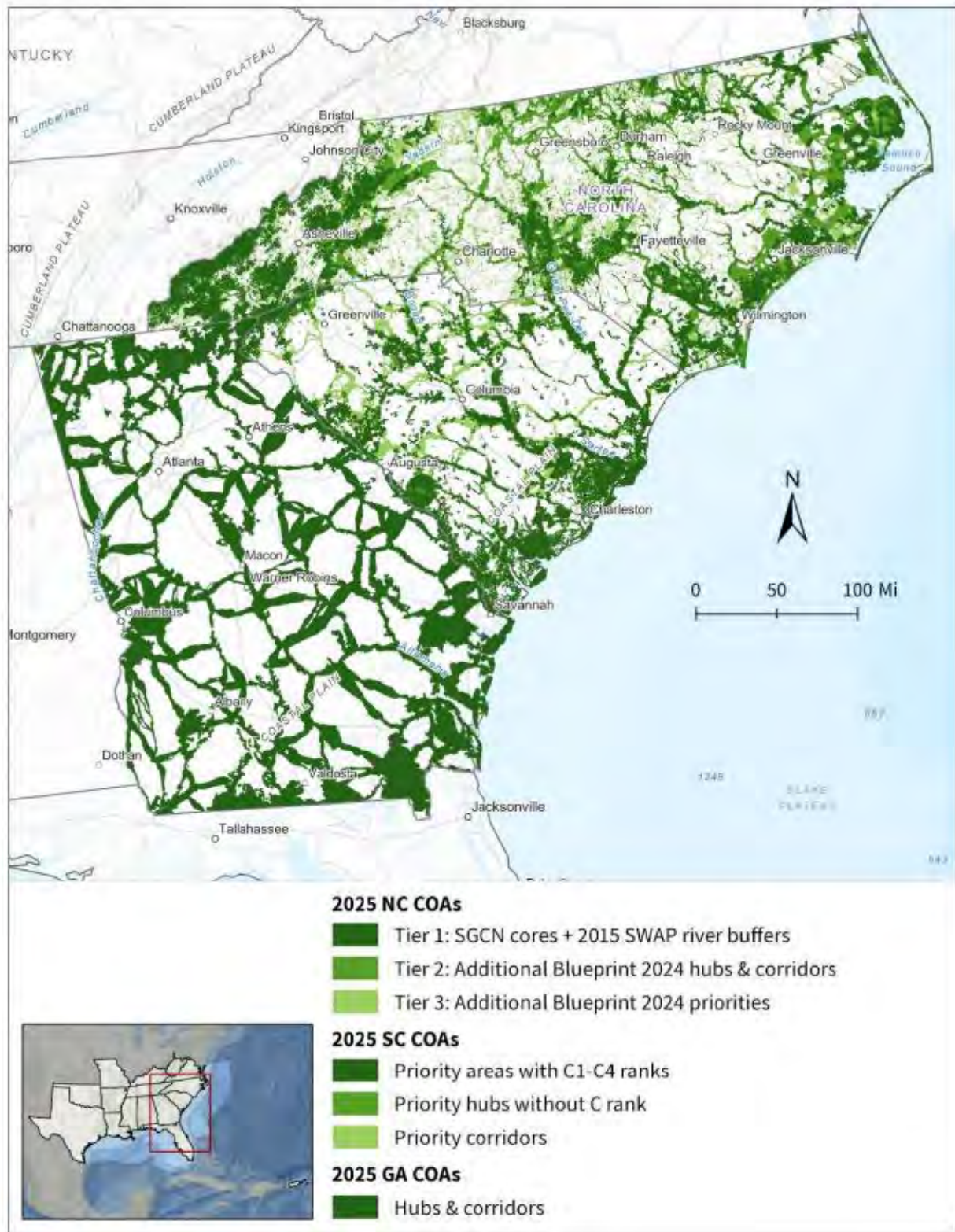
Figure 6.3-1. Map depicting NC and adjacent state COAs developed by SECAS for 2025 SWAPs.
