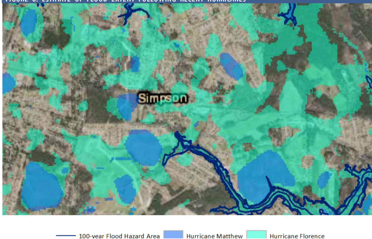
FIGURE 8. ESTIMATE OF FLOOD EXTENT FOLLOWING RECENT HURRICANES
